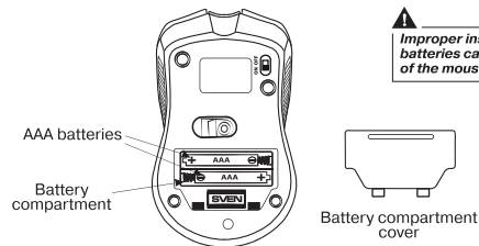
Fig. 4. Battery installation
